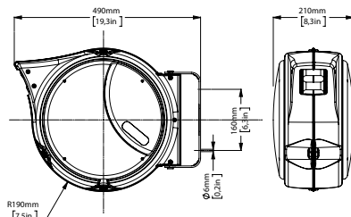
dimensions AM85
